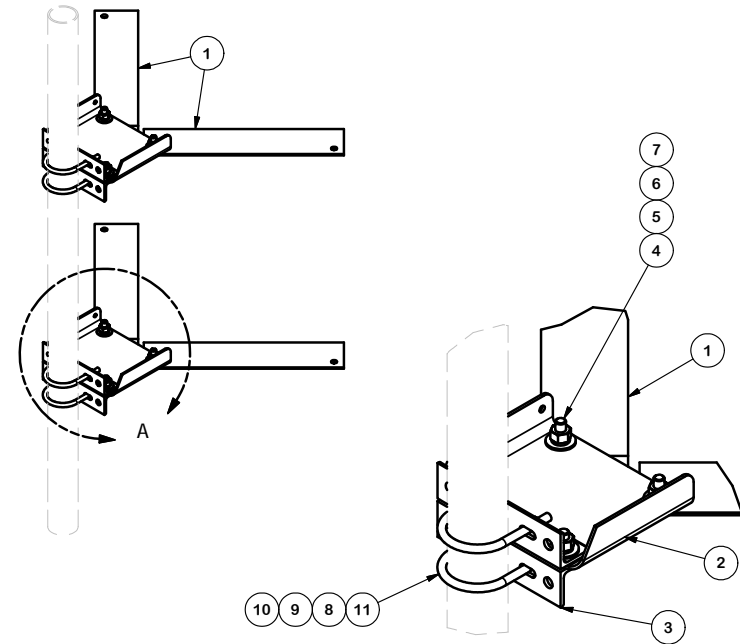
DETAIL A
